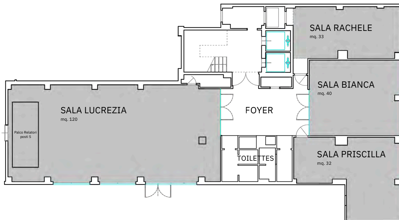
Basement Floor
